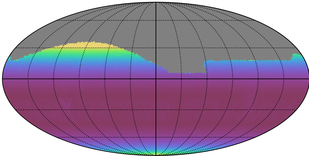
too_10_1v3.4_10yrs All sky g band: Min airmass
