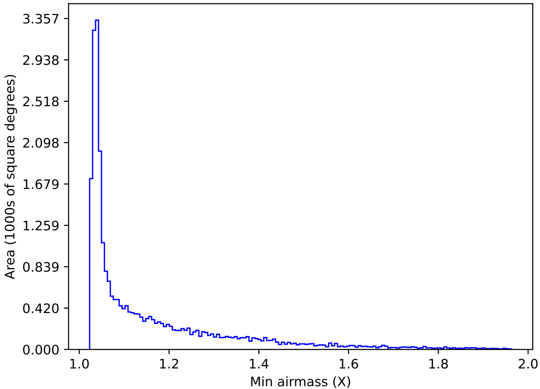
too_10_1v3.4_10yrs All sky g band: Min airmass
