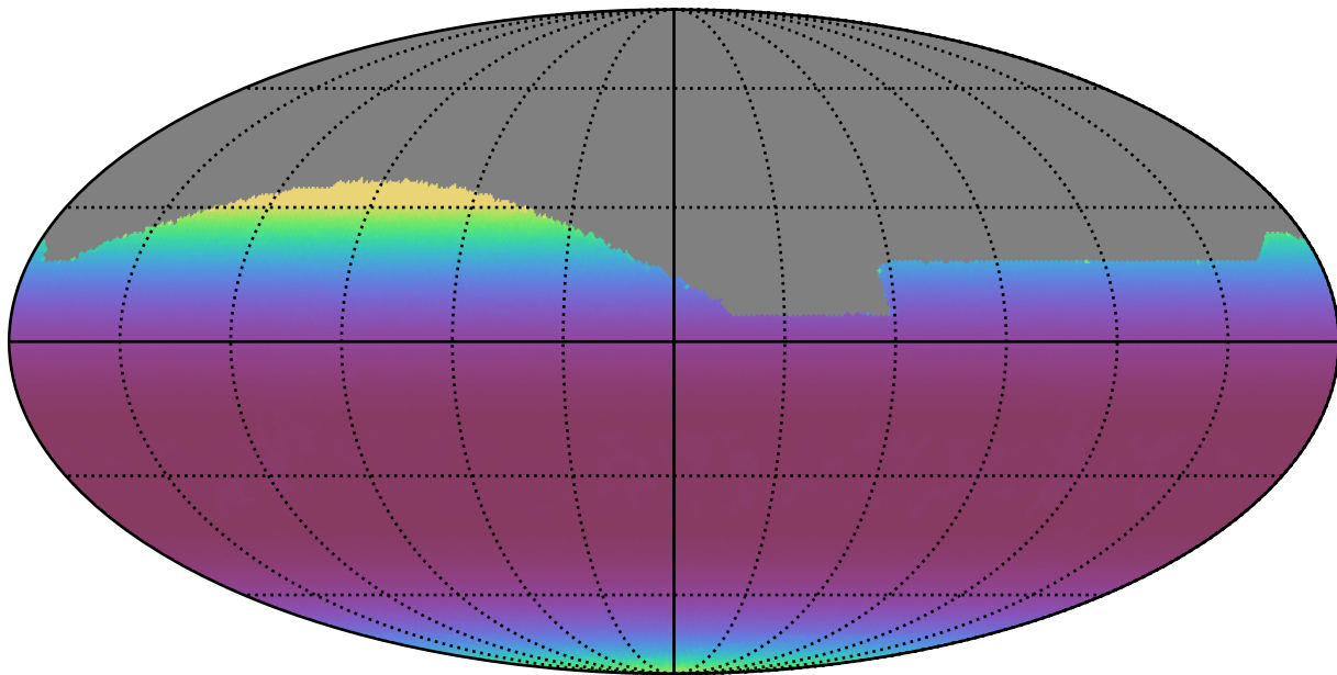
too_10_1v3.4_10yrs All sky all bands: Min airmass
