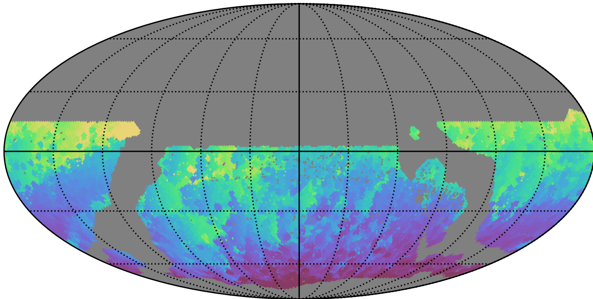
too_10_1v3.4_10yrs WFD z band: Min HA
