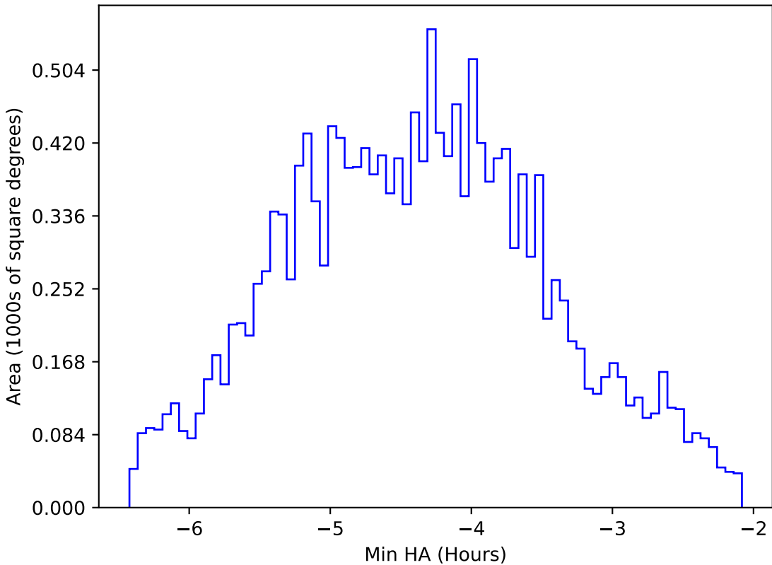
too_10_1v3.4_10yrs WFD z band: Min HA
