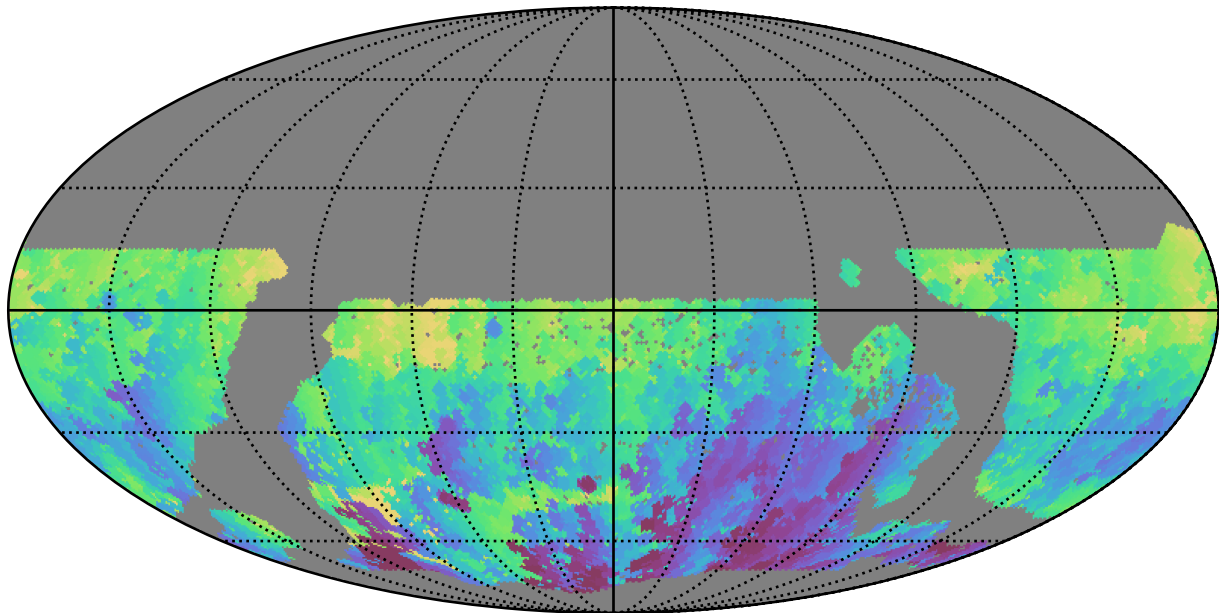
too_10_1v3.4_10yrs WFD u band: Min HA
