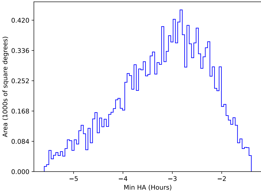
too_10_1v3.4_10yrs WFD u band: Min HA
