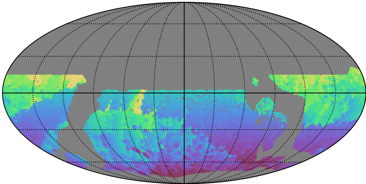
too_10_1v3.4_10yrs WFD r band: Min HA
