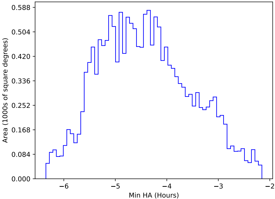
too_10_1v3.4_10yrs WFD r band: Min HA
