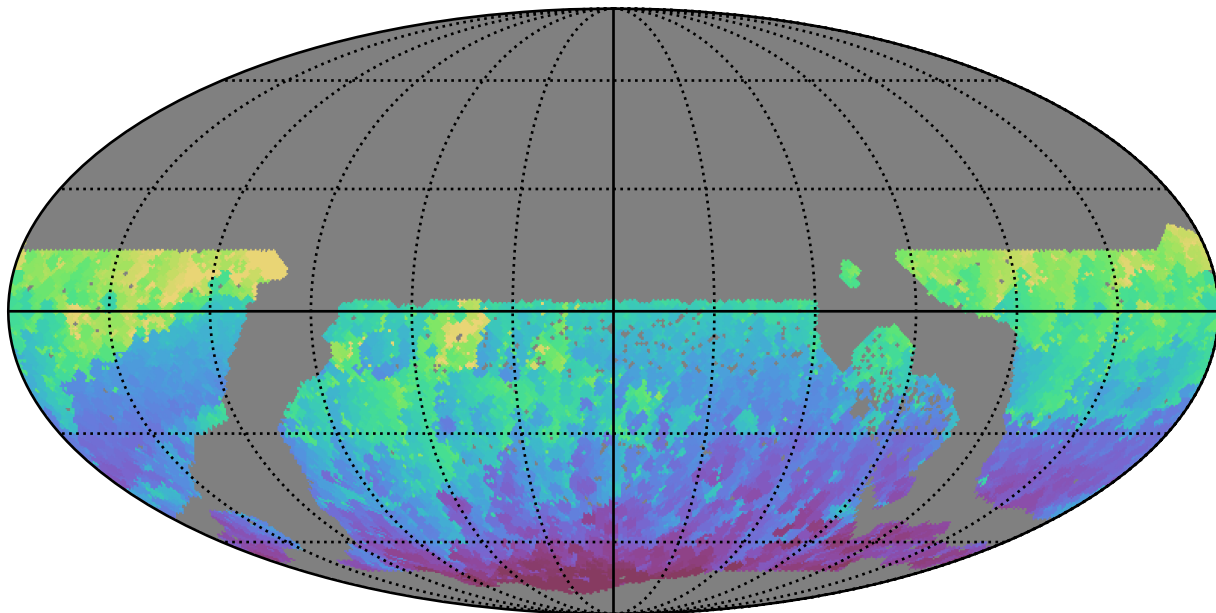
too_10_1v3.4_10yrs WFD i band: Min HA
