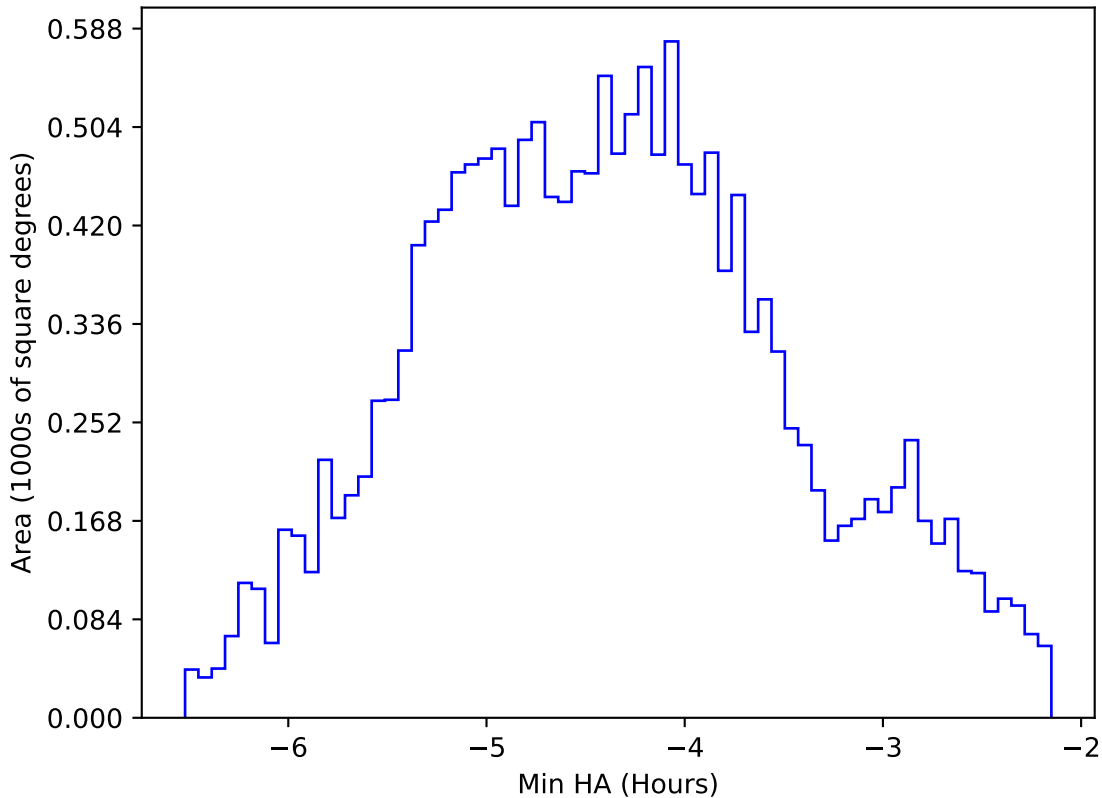
too_10_1v3.4_10yrs WFD i band: Min HA
