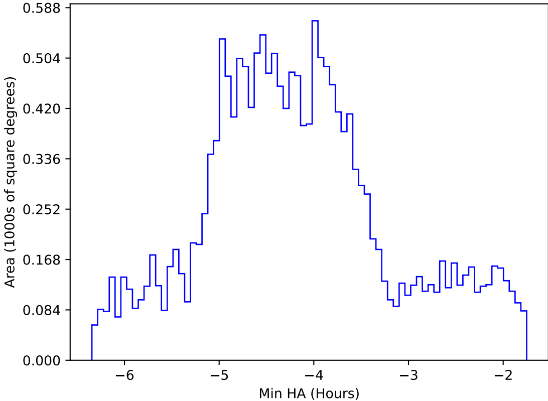
too_10_1v3.4_10yrs WFD g band: Min HA
