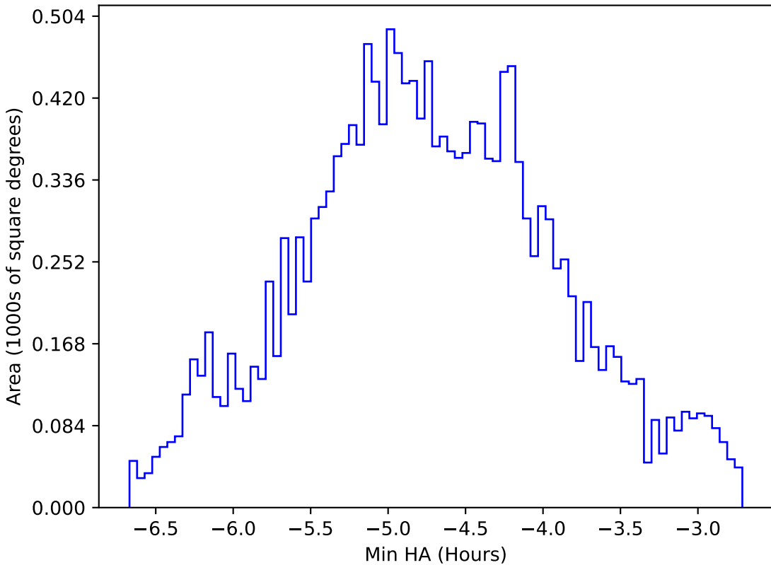
too_10_1v3.4_10yrs WFD all bands: Min HA
