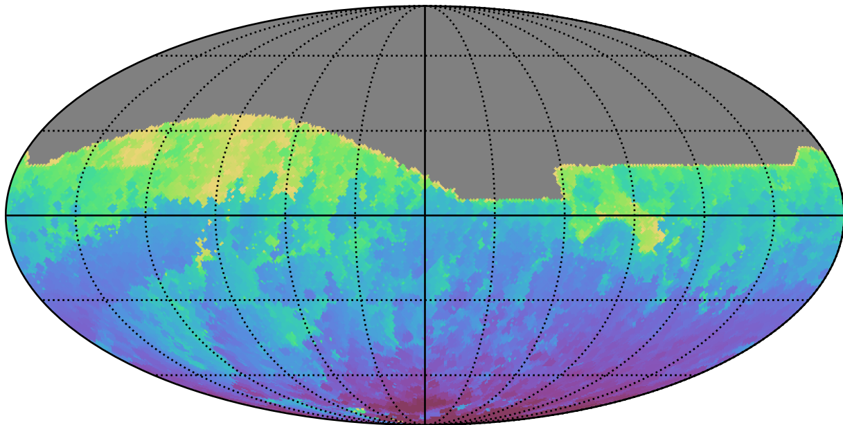
too_10_1v3.4_10yrs All sky z band: Min HA
