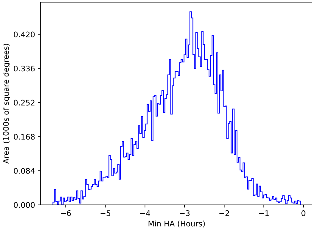
too_10_1v3.4_10yrs All sky u band: Min HA
