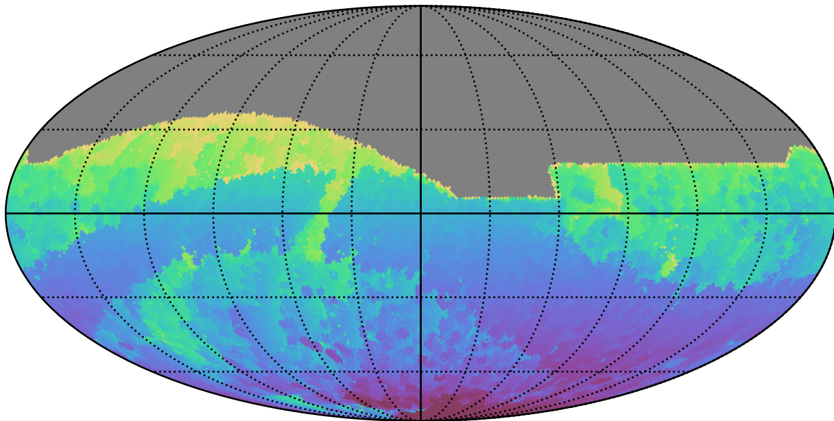
too_10_1v3.4_10yrs All sky r band: Min HA
