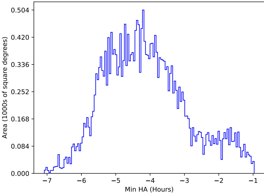
too_10_1v3.4_10yrs All sky r band: Min HA
