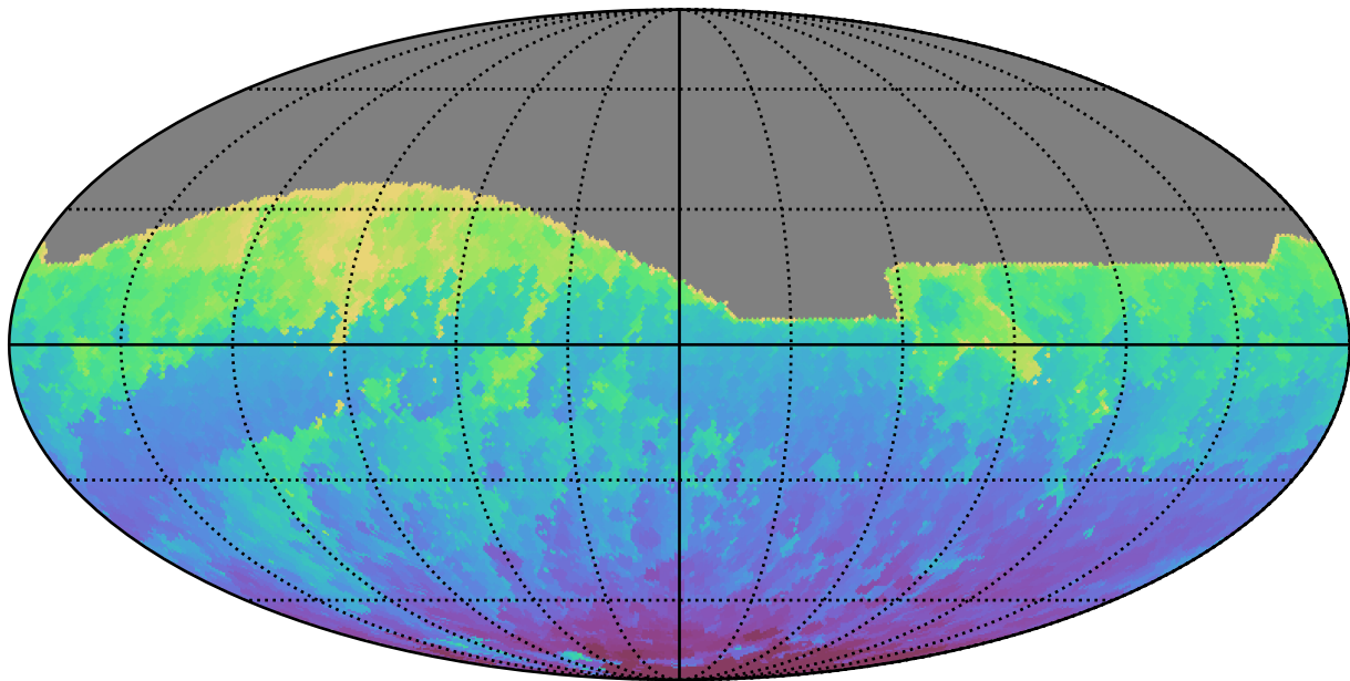
too_10_1v3.4_10yrs All sky i band: Min HA
