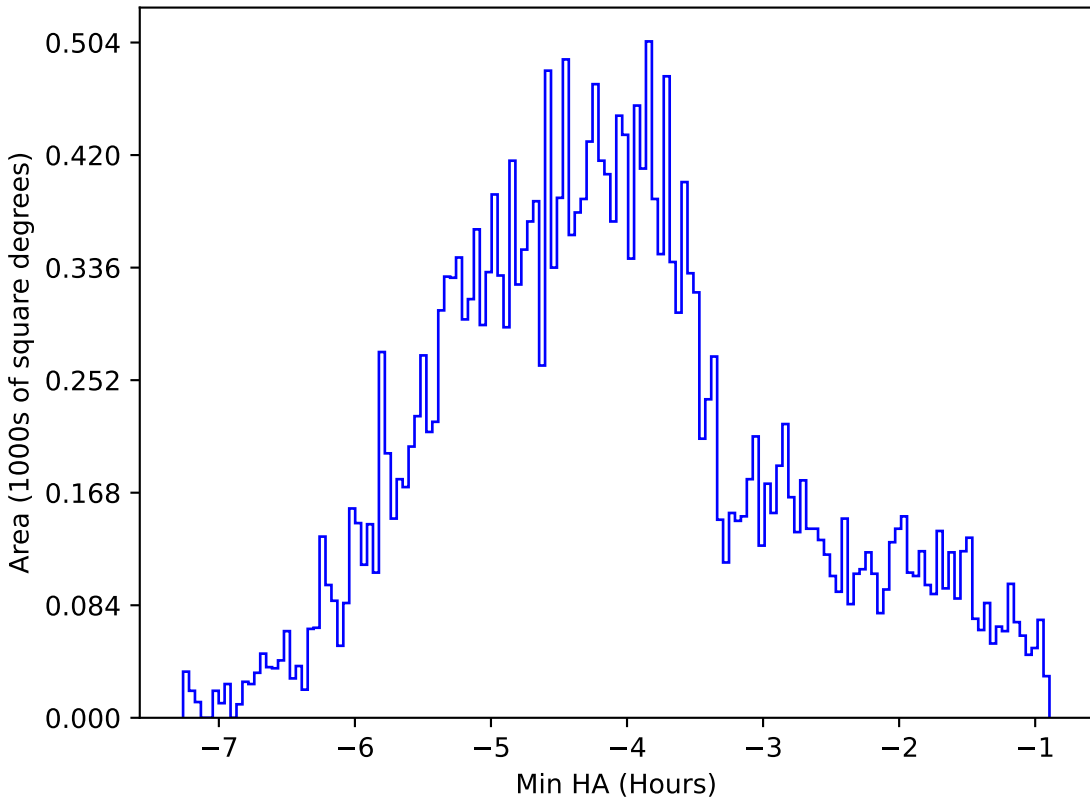
too_10_1v3.4_10yrs All sky i band: Min HA
