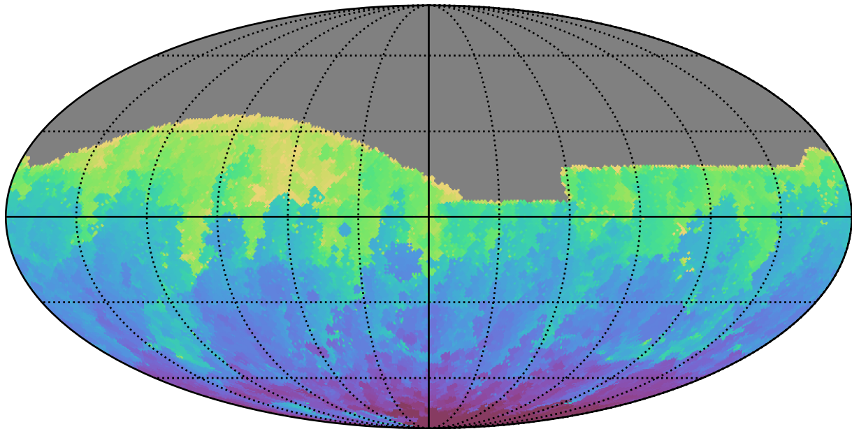
too_10_1v3.4_10yrs All sky g band: Min HA
