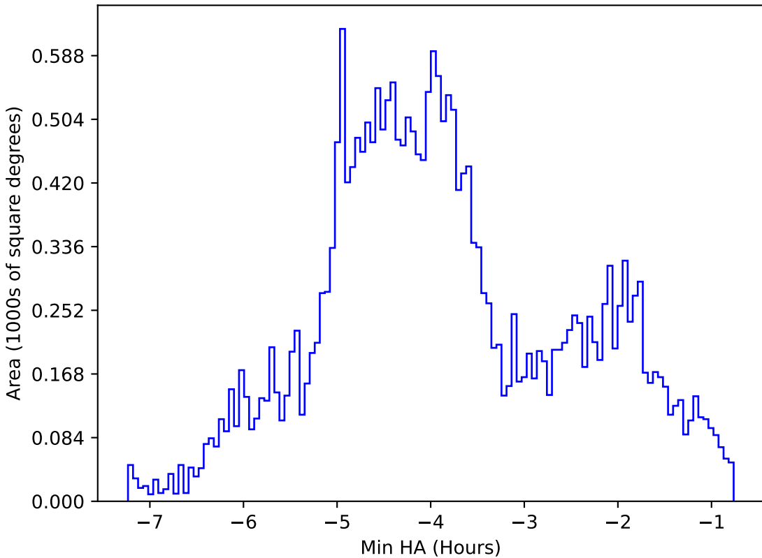
too_10_1v3.4_10yrs All sky g band: Min HA
