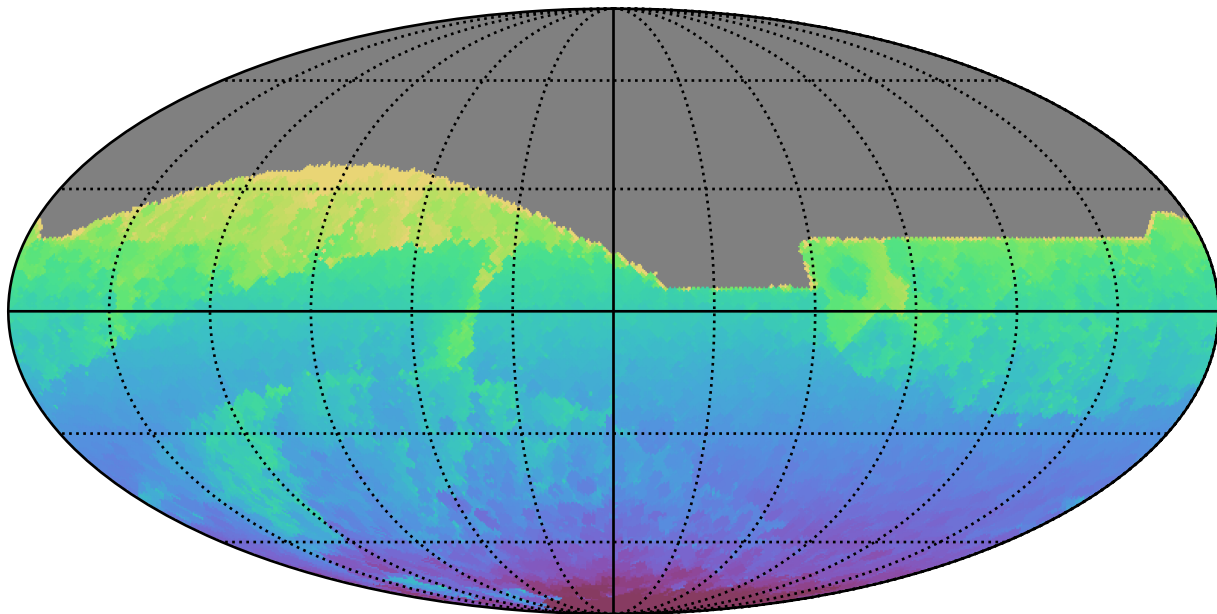
too_10_1v3.4_10yrs All sky all bands: Min HA
