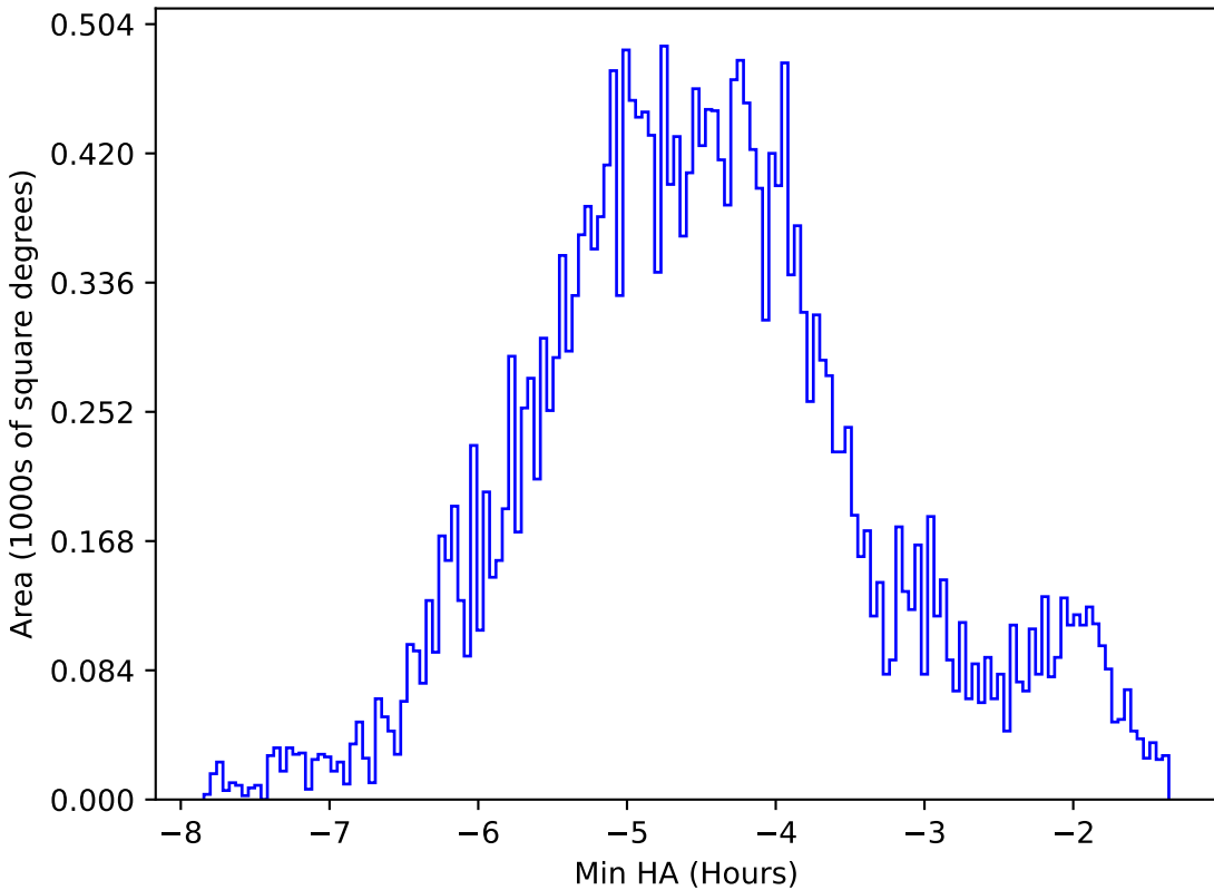
too_10_1v3.4_10yrs All sky all bands: Min HA
