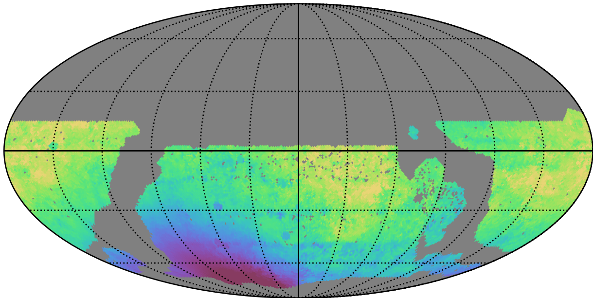
too_10_1v3.4_10yrs WFD z band: Median solarElong
