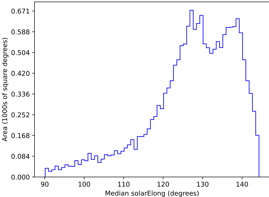
too_10_1v3.4_10yrs WFD z band: Median solarElong
