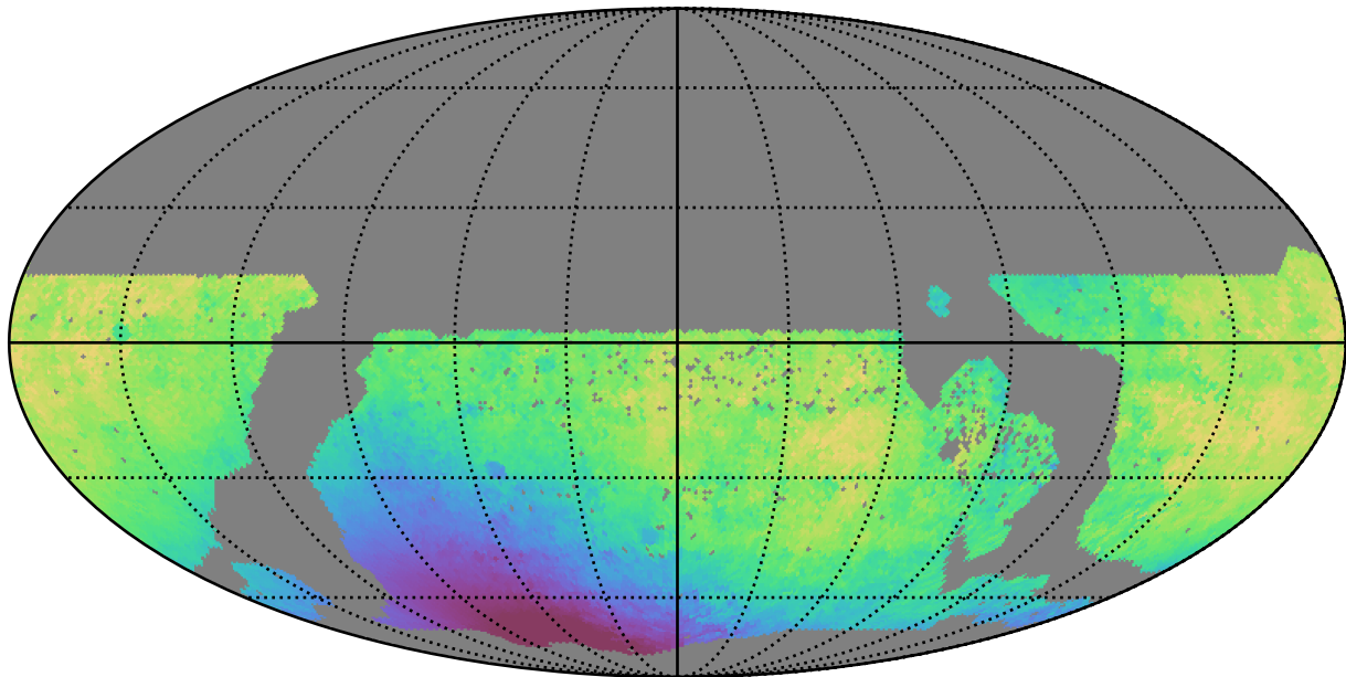
too_10_1v3.4_10yrs WFD y band: Median solarElong
