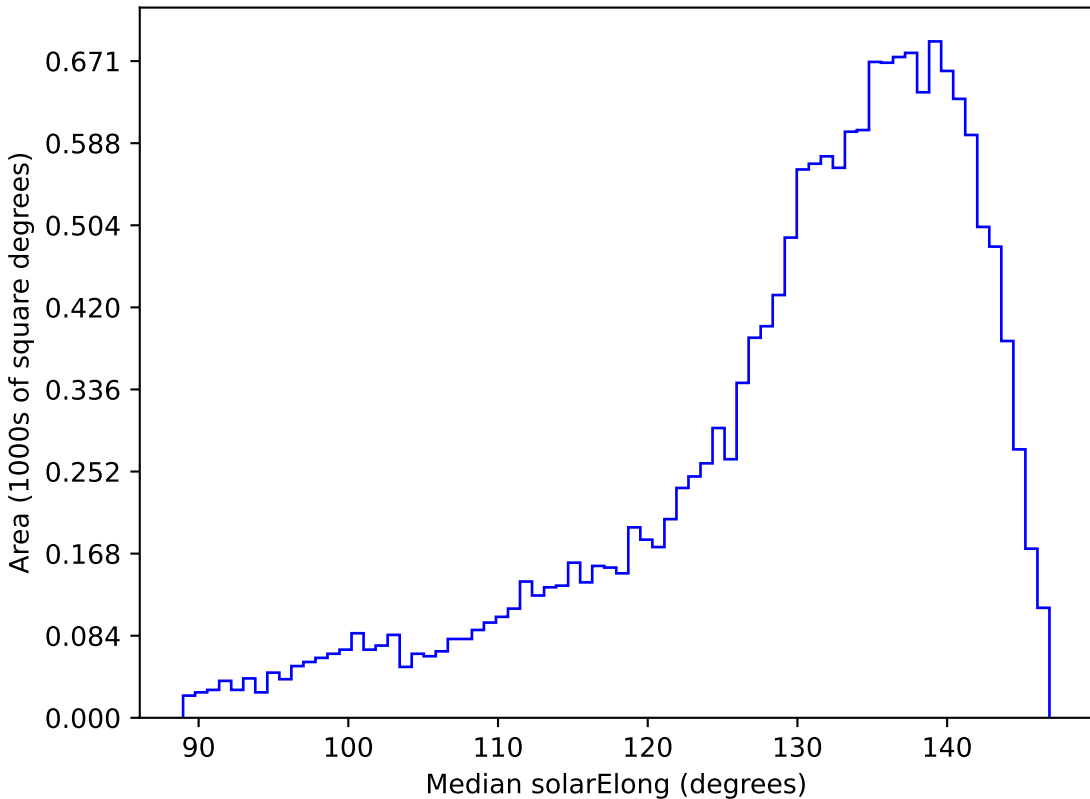
too_10_1v3.4_10yrs WFD y band: Median solarElong
