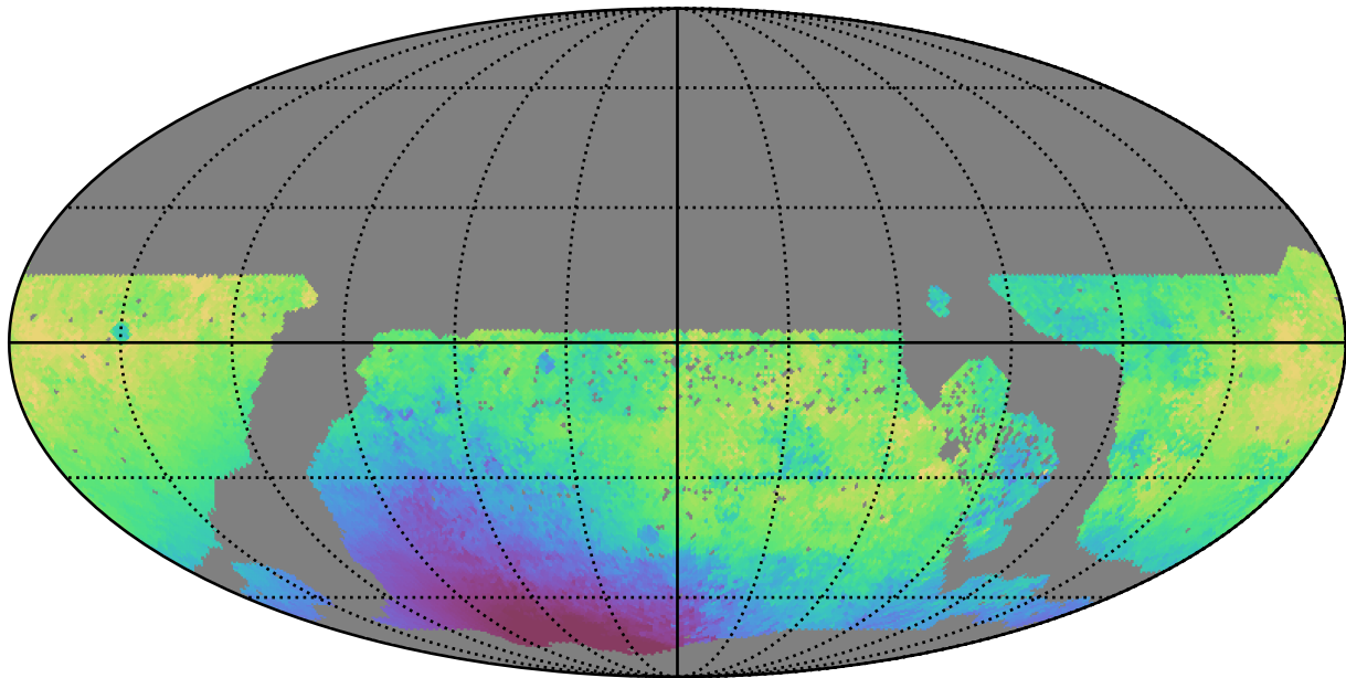
too_10_1v3.4_10yrs WFD u band: Median solarElong
