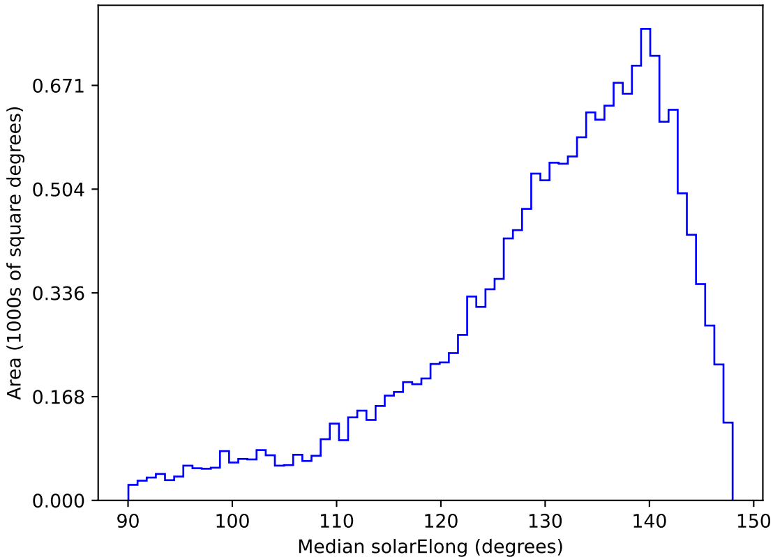
too_10_1v3.4_10yrs WFD r band: Median solarElong
