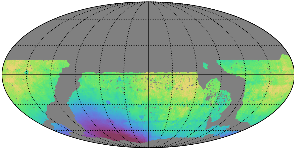
too_10_1v3.4_10yrs WFD i band: Median solarElong
