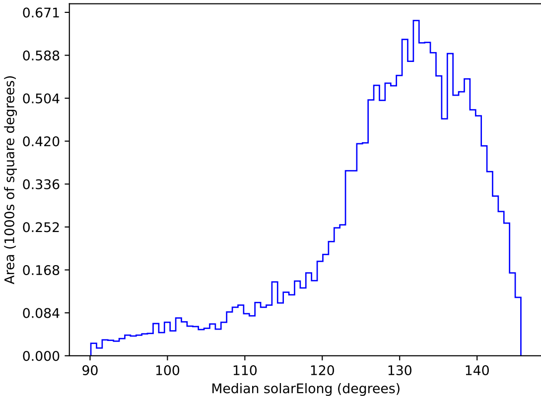
too_10_1v3.4_10yrs WFD i band: Median solarElong
