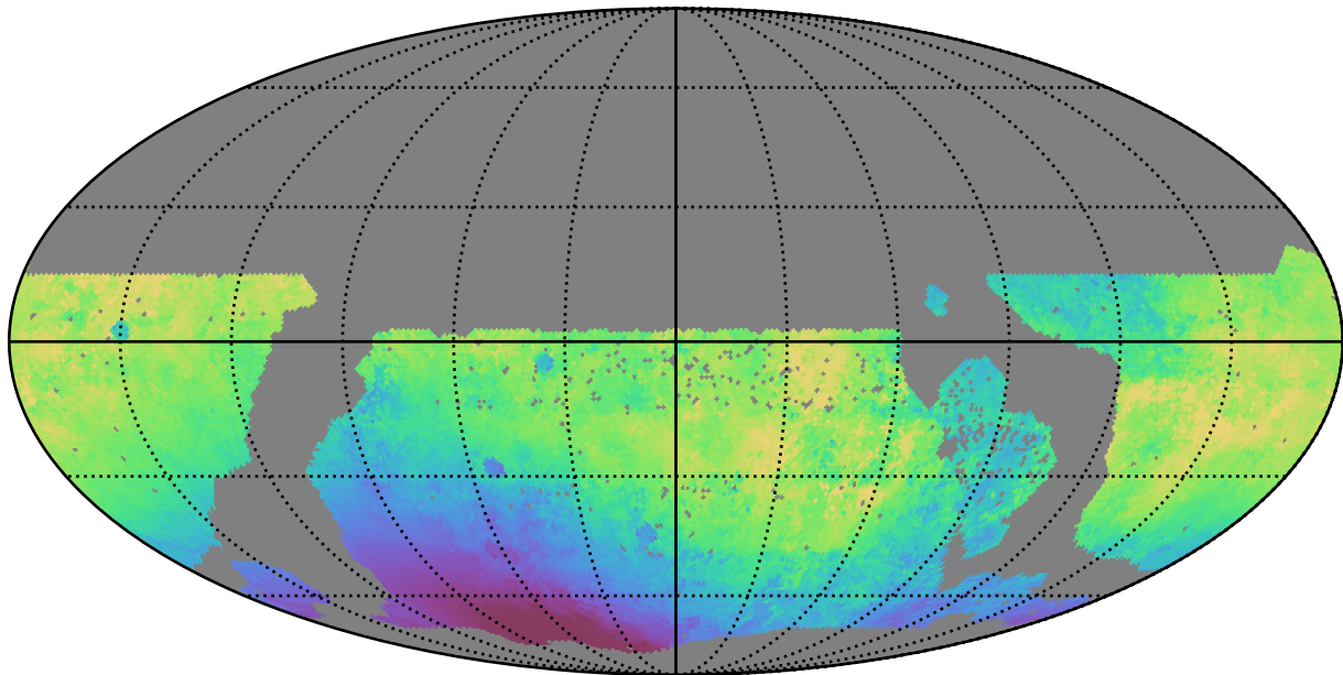
too_10_1v3.4_10yrs WFD g band: Median solarElong
