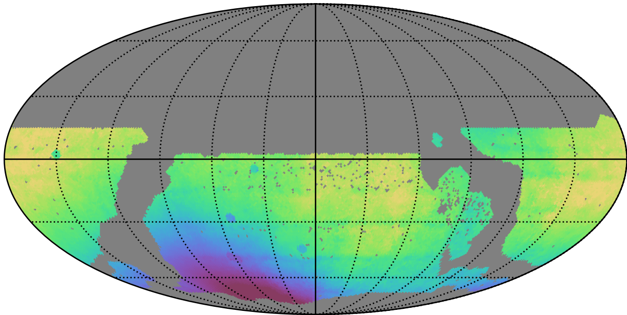
too_10_1v3.4_10yrs WFD all bands: Median solarElong
