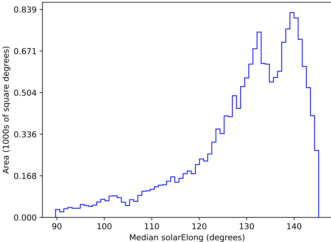
too_10_1v3.4_10yrs WFD all bands: Median solarElong
