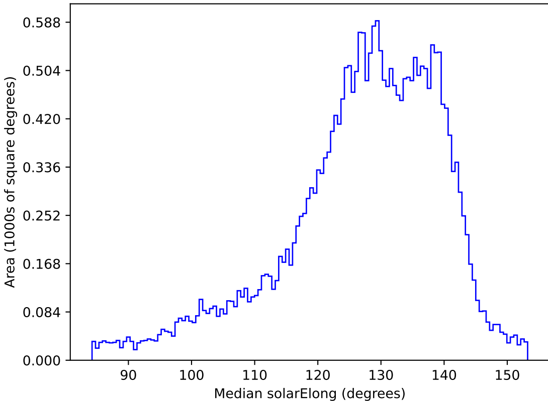
too_10_1v3.4_10yrs All sky z band: Median solarElong
