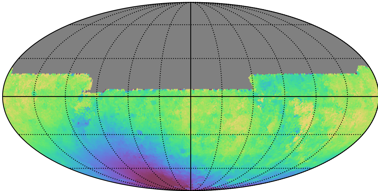
too_10_1v3.4_10yrs All sky y band: Median solarElong
