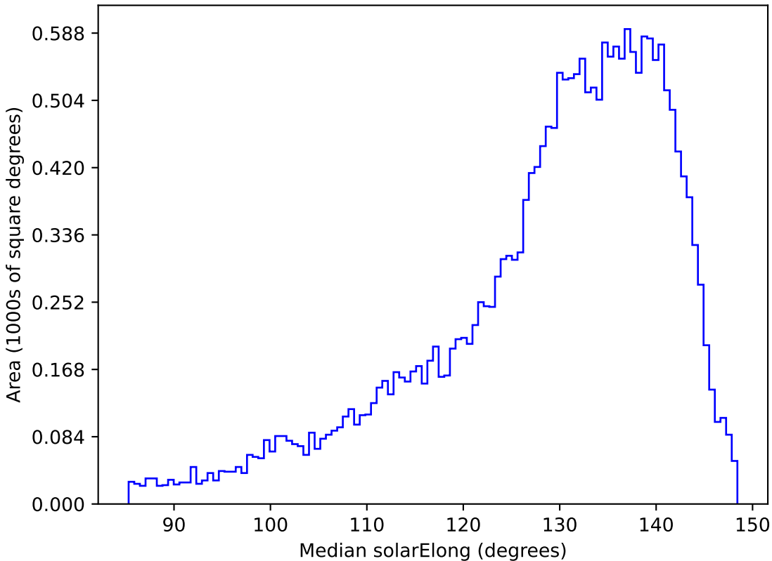
too_10_1v3.4_10yrs All sky y band: Median solarElong
