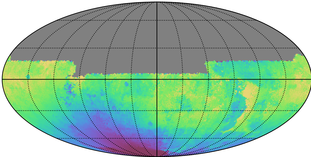
too_10_1v3.4_10yrs All sky u band: Median solarElong
