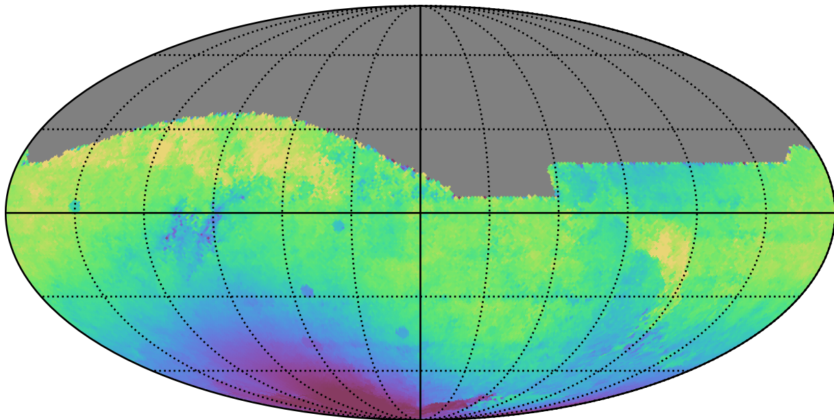
too_10_1v3.4_10yrs All sky r band: Median solarElong
