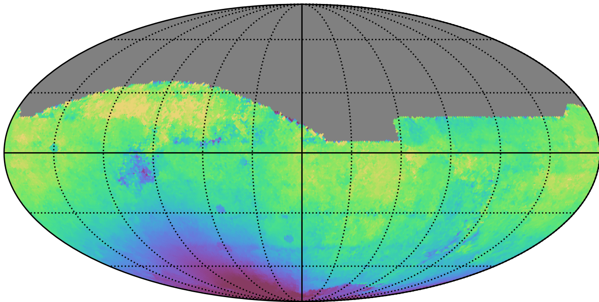
too_10_1v3.4_10yrs All sky i band: Median solarElong
