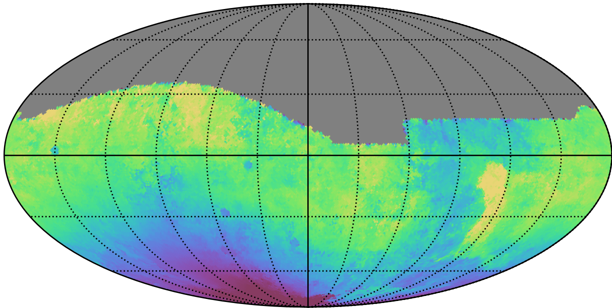
too_10_1v3.4_10yrs All sky g band: Median solarElong
