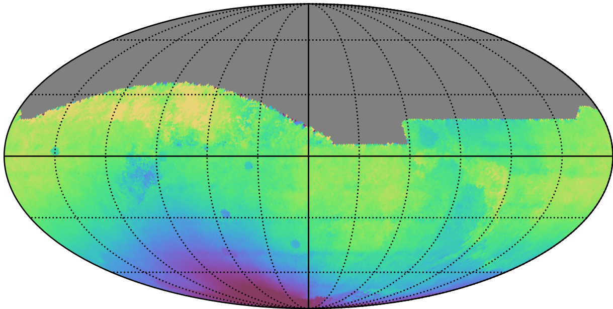
too_10_1v3.4_10yrs All sky all bands: Median solarElong
