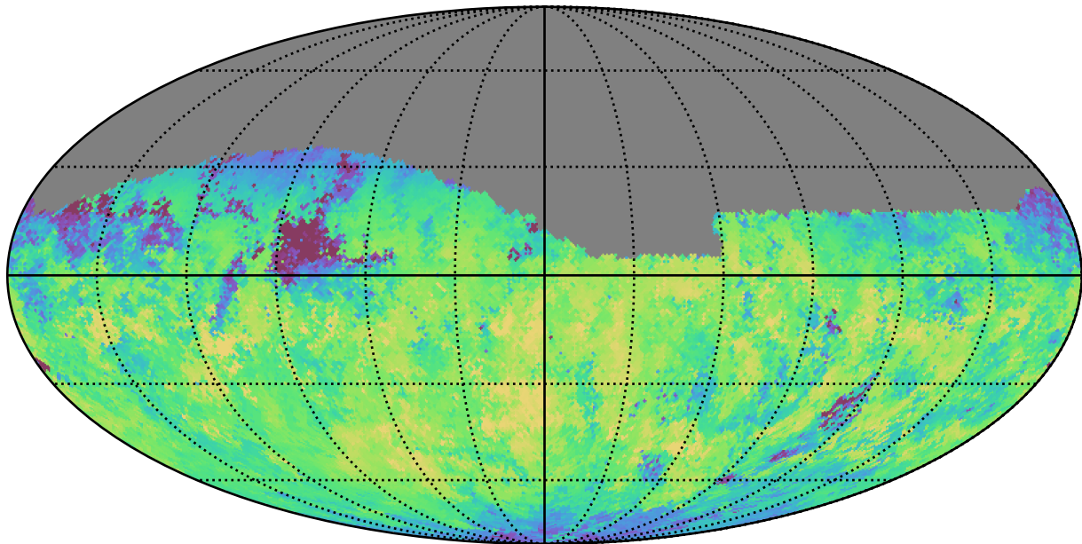
too_10_1v3.4_10yrs Yr 1 z band: Median skyBrightness
