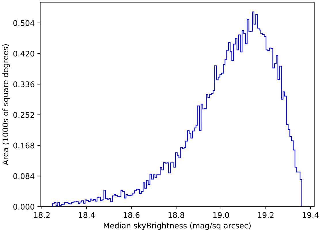
too_10_1v3.4_10yrs Yr 1 z band: Median skyBrightness
