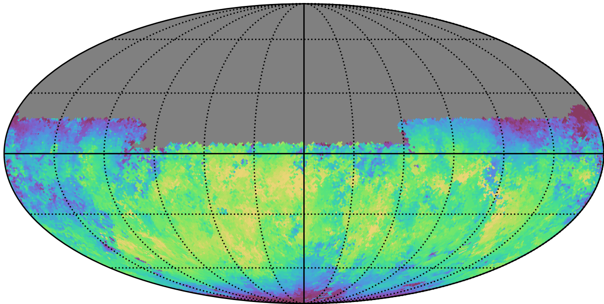
too_10_1v3.4_10yrs Yr 1 y band: Median skyBrightness
