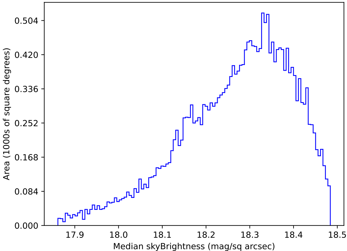
too_10_1v3.4_10yrs Yr 1 y band: Median skyBrightness
