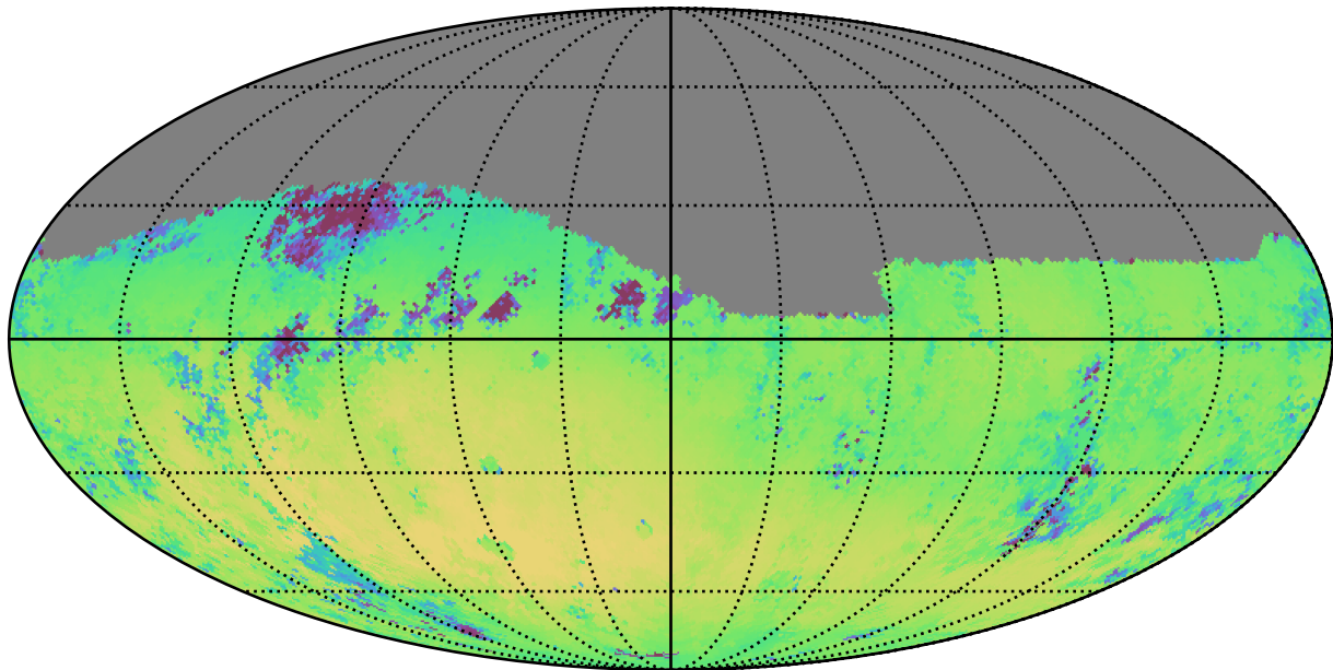
too_10_1v3.4_10yrs Yr 1 r band: Median skyBrightness
