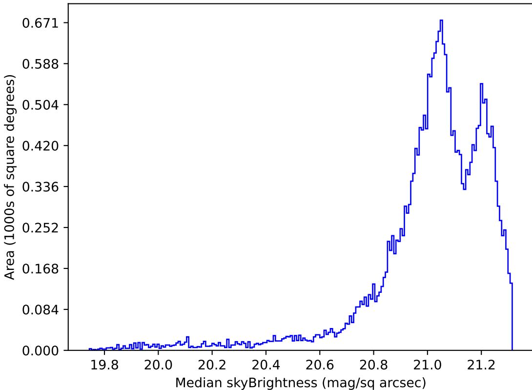
too_10_1v3.4_10yrs Yr 1 r band: Median skyBrightness
