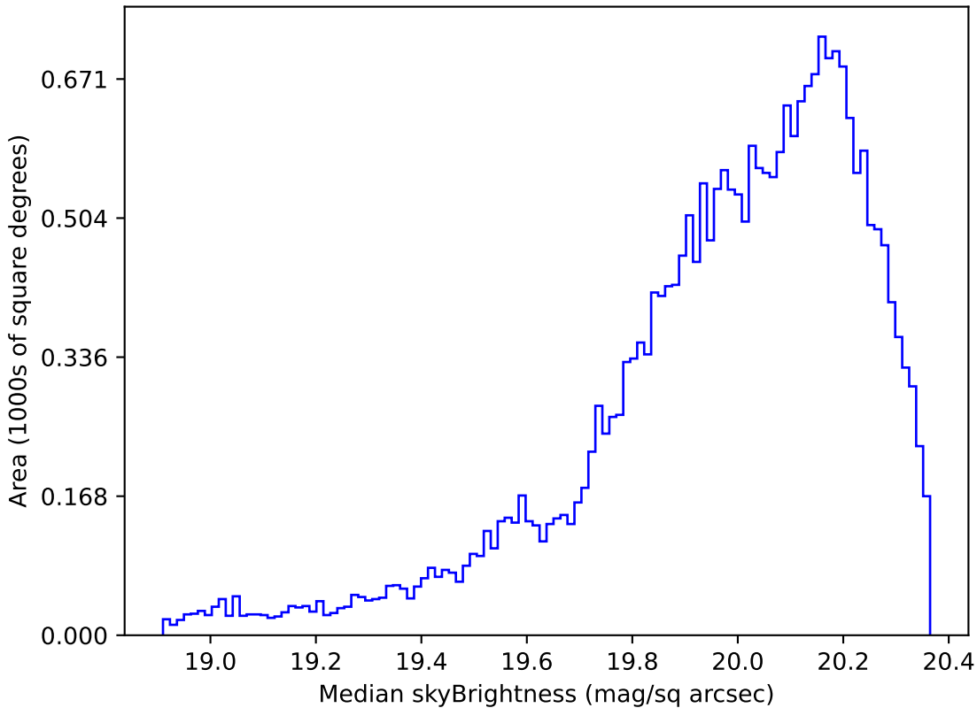
too_10_1v3.4_10yrs Yr 1 i band: Median skyBrightness
