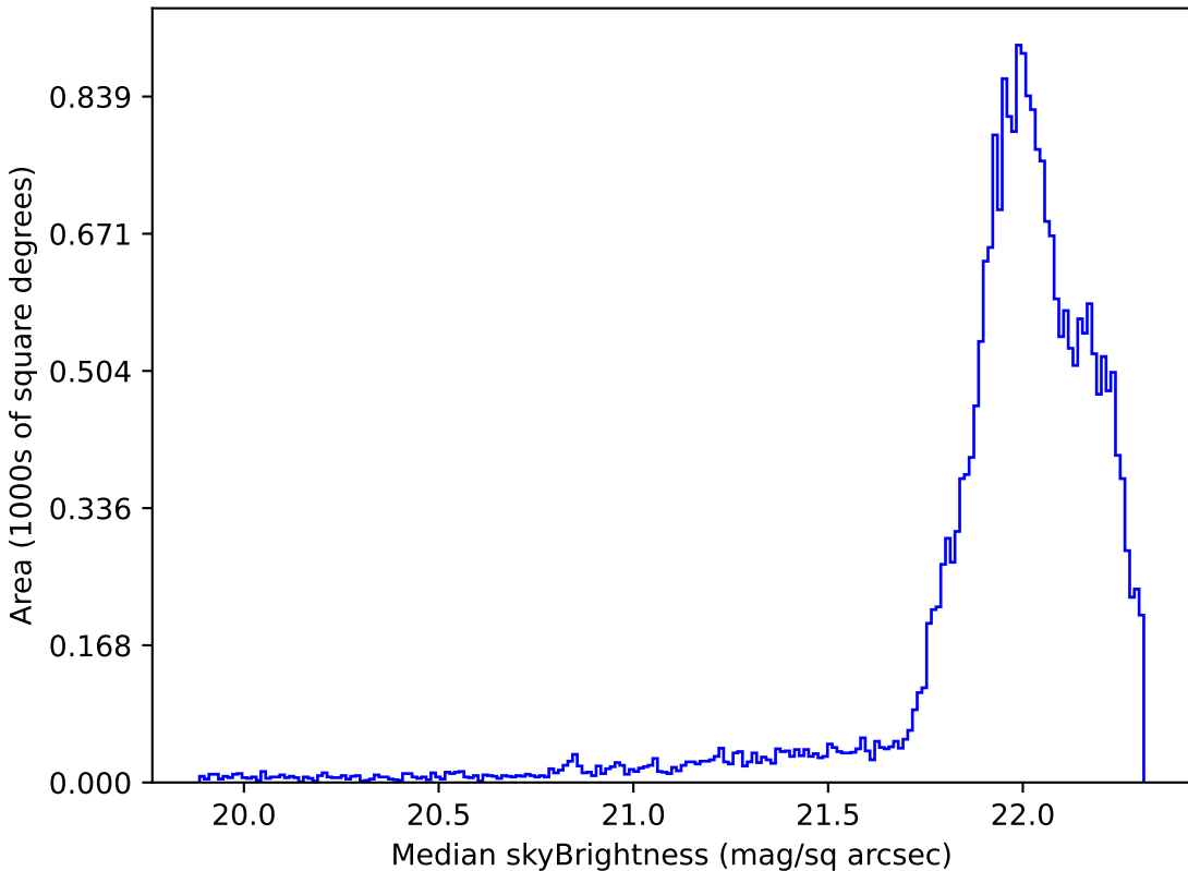
too_10_1v3.4_10yrs Yr 1 g band: Median skyBrightness
